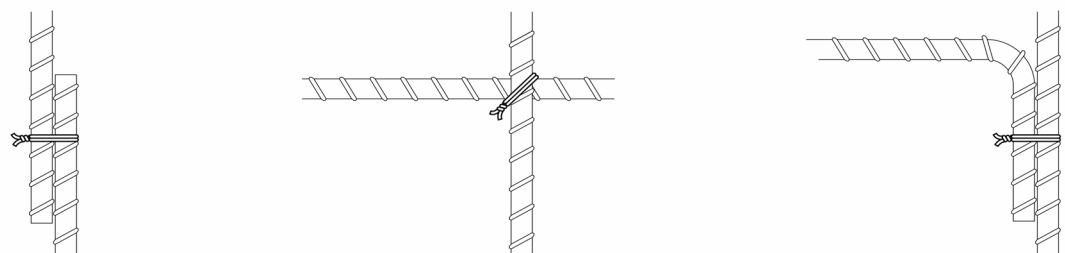
Figure E.5c – Bound joints (suitable for lightning current and EMC purposes)
