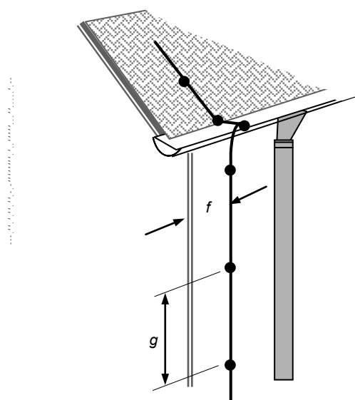
Figure E.22c – Installation of a down-conductor with connection to the gutter
