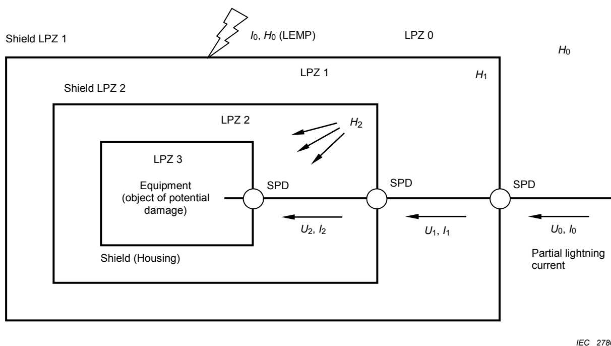
Figure A.1 – LEMP situation due to lightning strike
