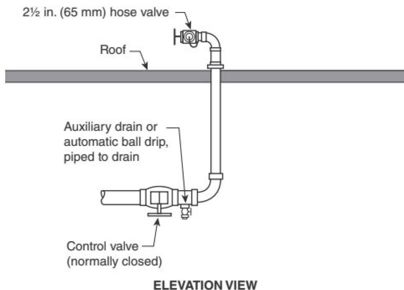
FIGURE A.9.5.2.6.4(b) Roof Hose Connection Piping.
