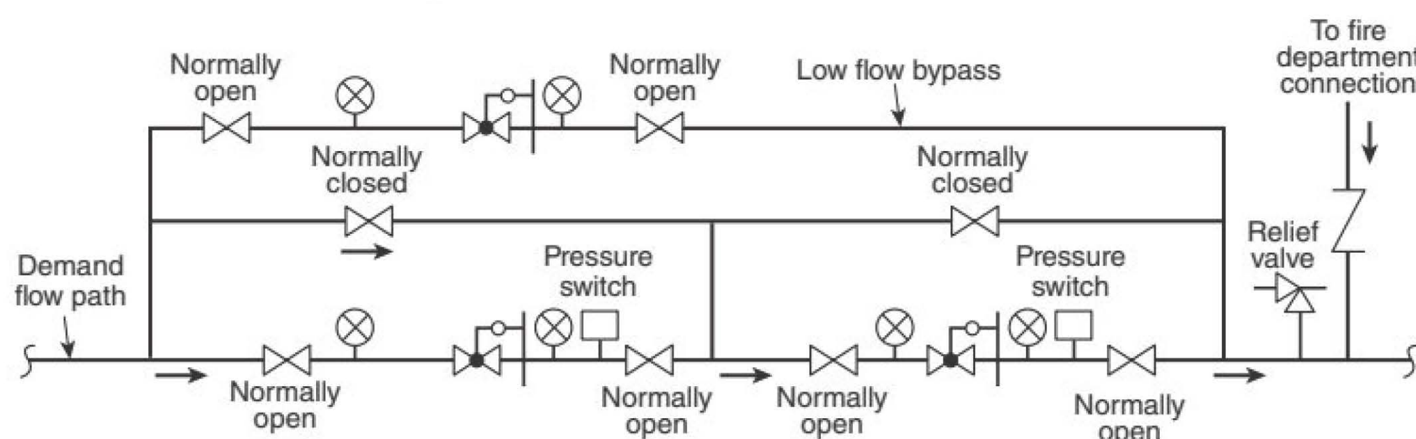
FIGURE A.10.2.5(a) Dual Pressure-Regulating Device Arrangement.
