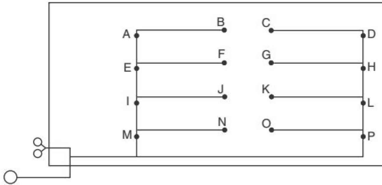
FIGURE A.10.6.1.1.7 Standpipe System with Single Hose Connections Served by a Lateral Pipe.
