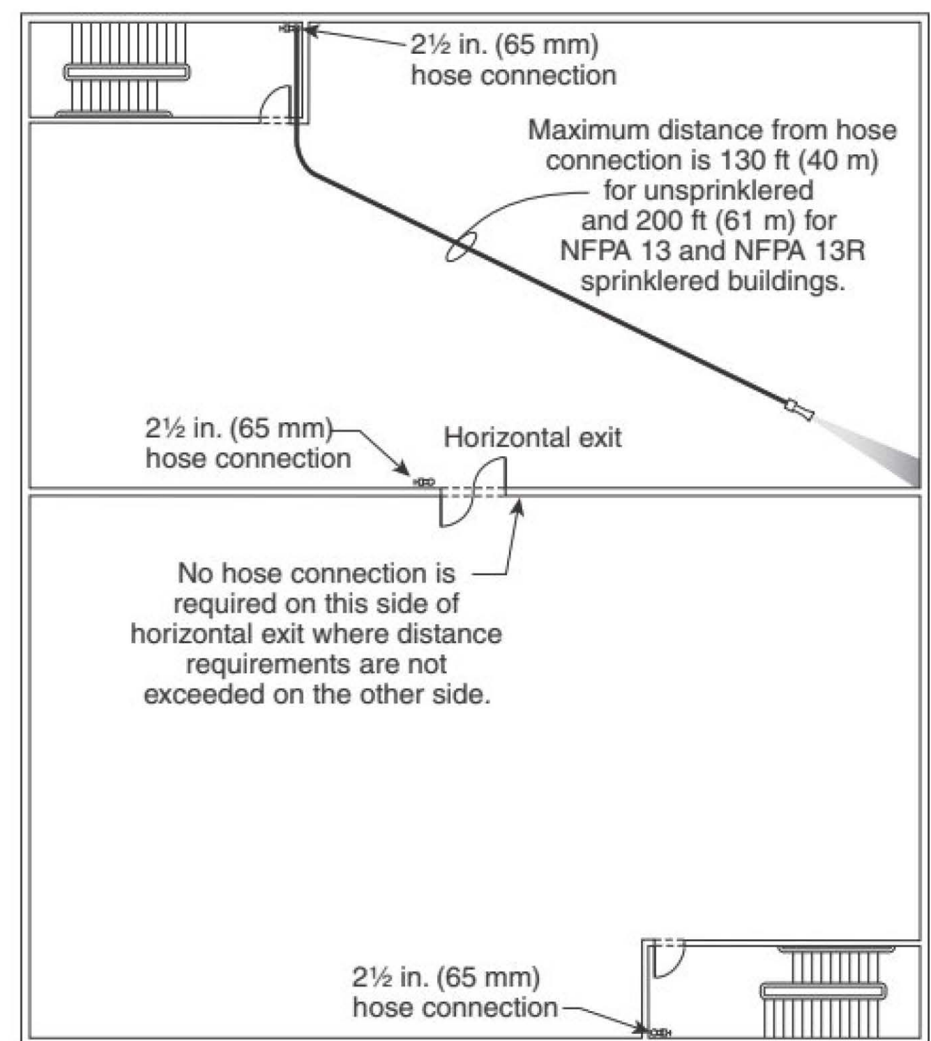
FIGURE A.9.5.2.2.1 Location of Hose Connections at Horizontal Exits and Stairwells.
