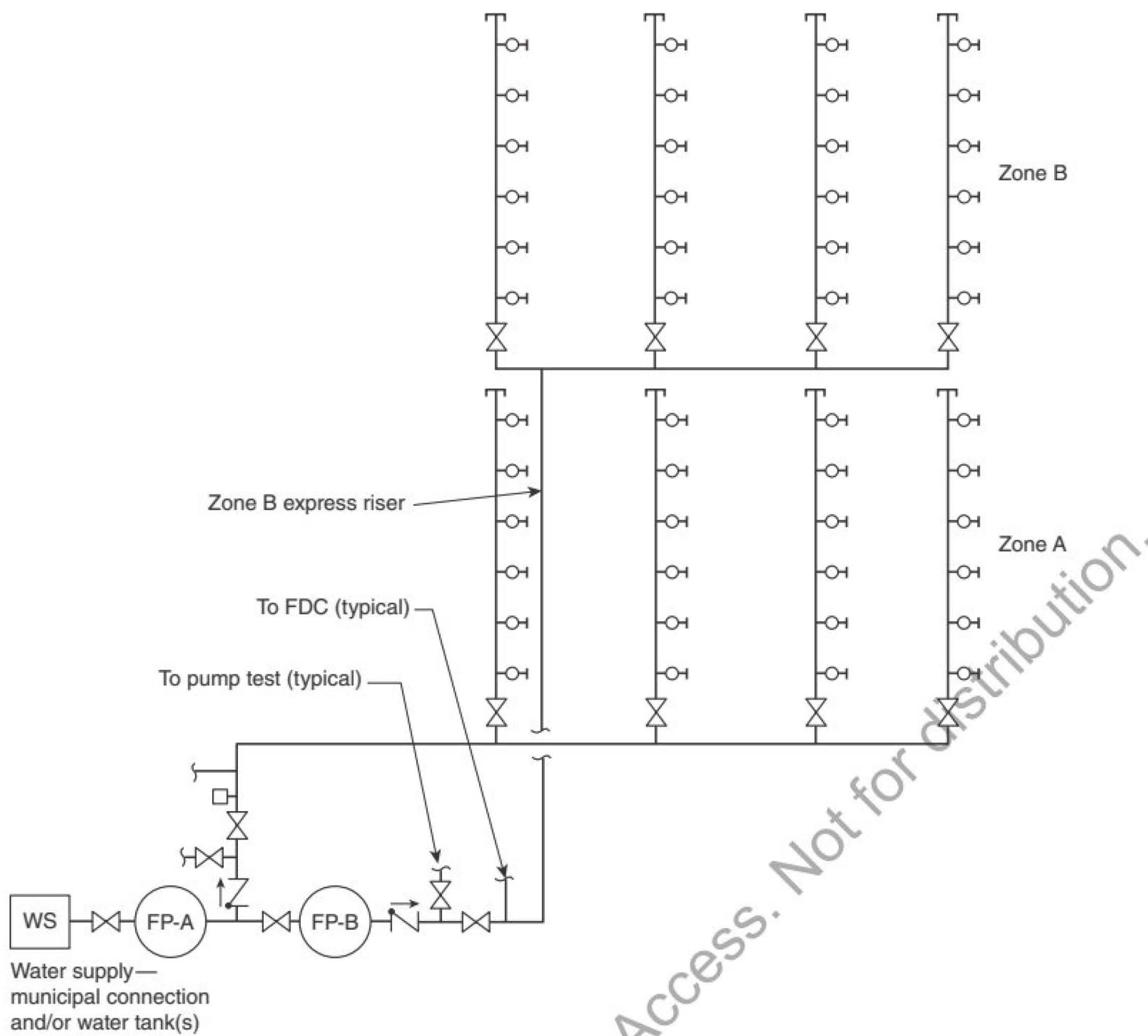
FIGURE A.10.5.2(n) Zones Up to the Level of Fire Department Pumping Capacity Using Pumps in Series — Two Vertical Standpipe System Zones Example.
