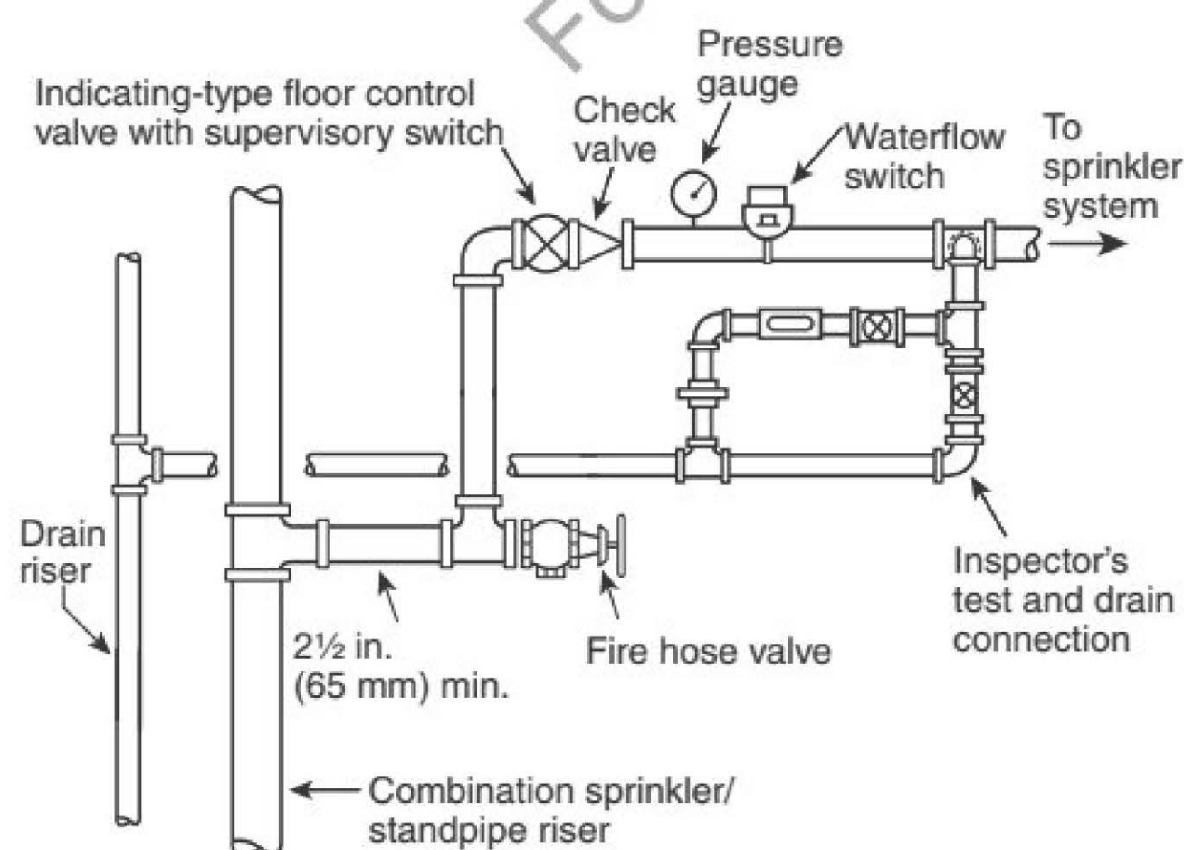
FIGURE A.9.6.6(b) Combined Sprinkler/Standpipe System.
