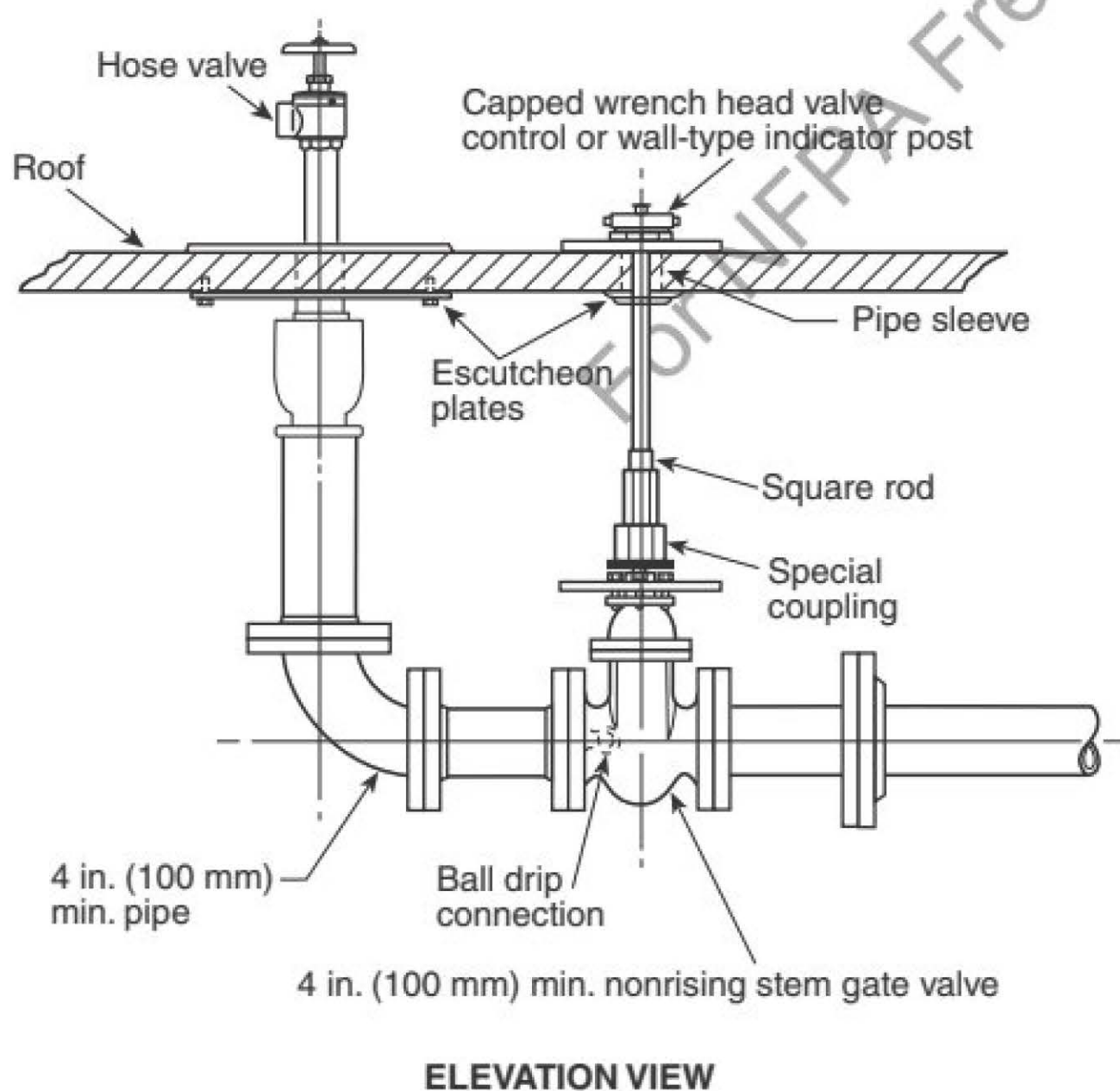
FIGURE A.9.5.2.6.4(a) Roof Hose Connection Piping Arrangement.
