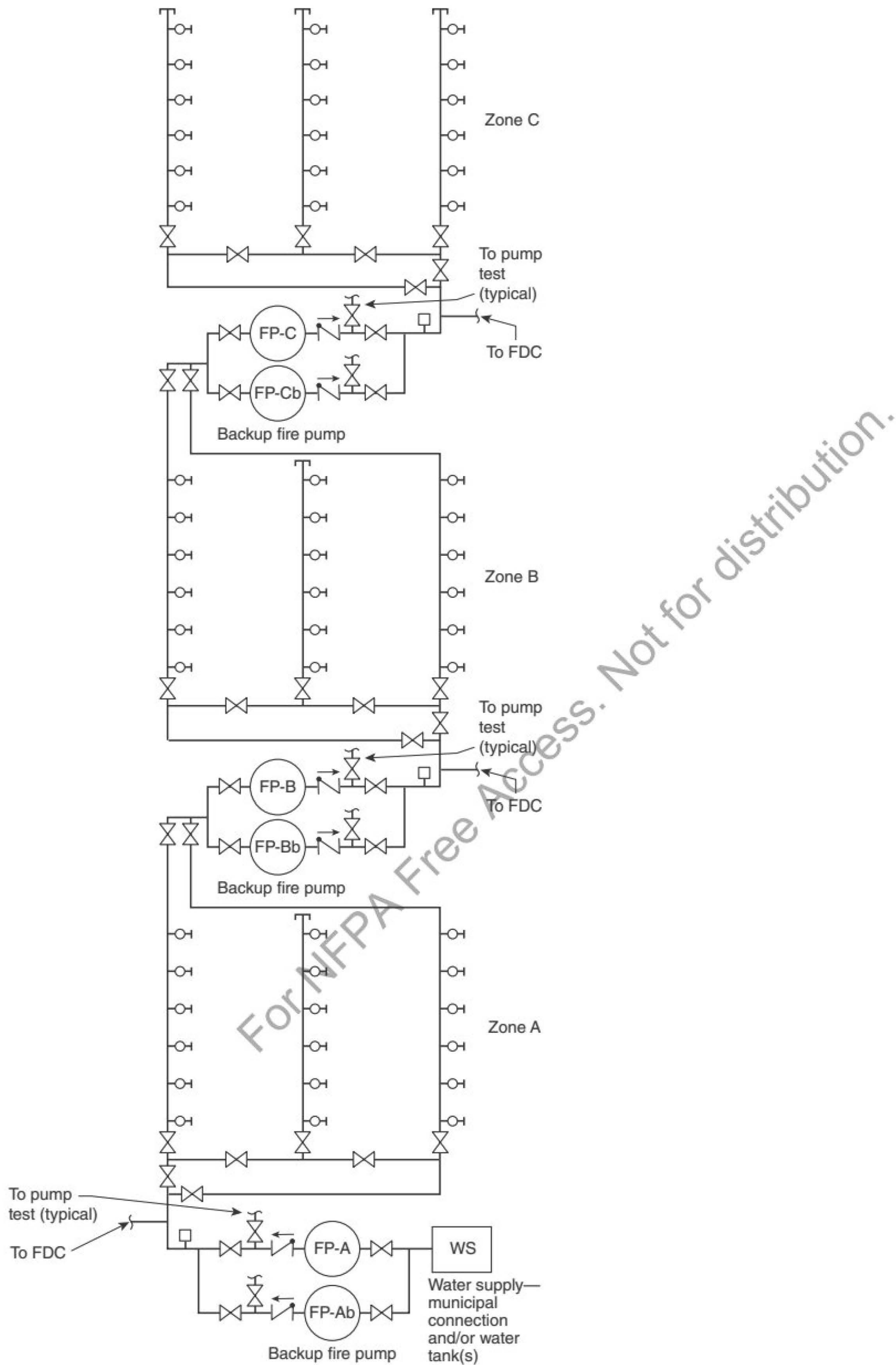
FIGURE A.10.5.3(m) Zones Partially or Wholly Above the Level of Fire Department Pumping Capacity — Vertically Staged Fire Pumps with Pump Suction Supply Risers Using Standpipe Risers — Three Vertical Standpipe System Zones Example.
