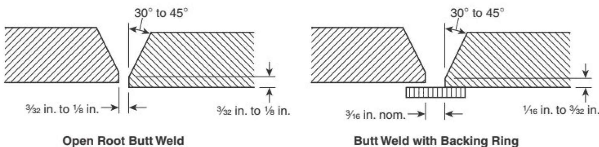
FIGURE A.7.4.2.2 Weld Diagram.
