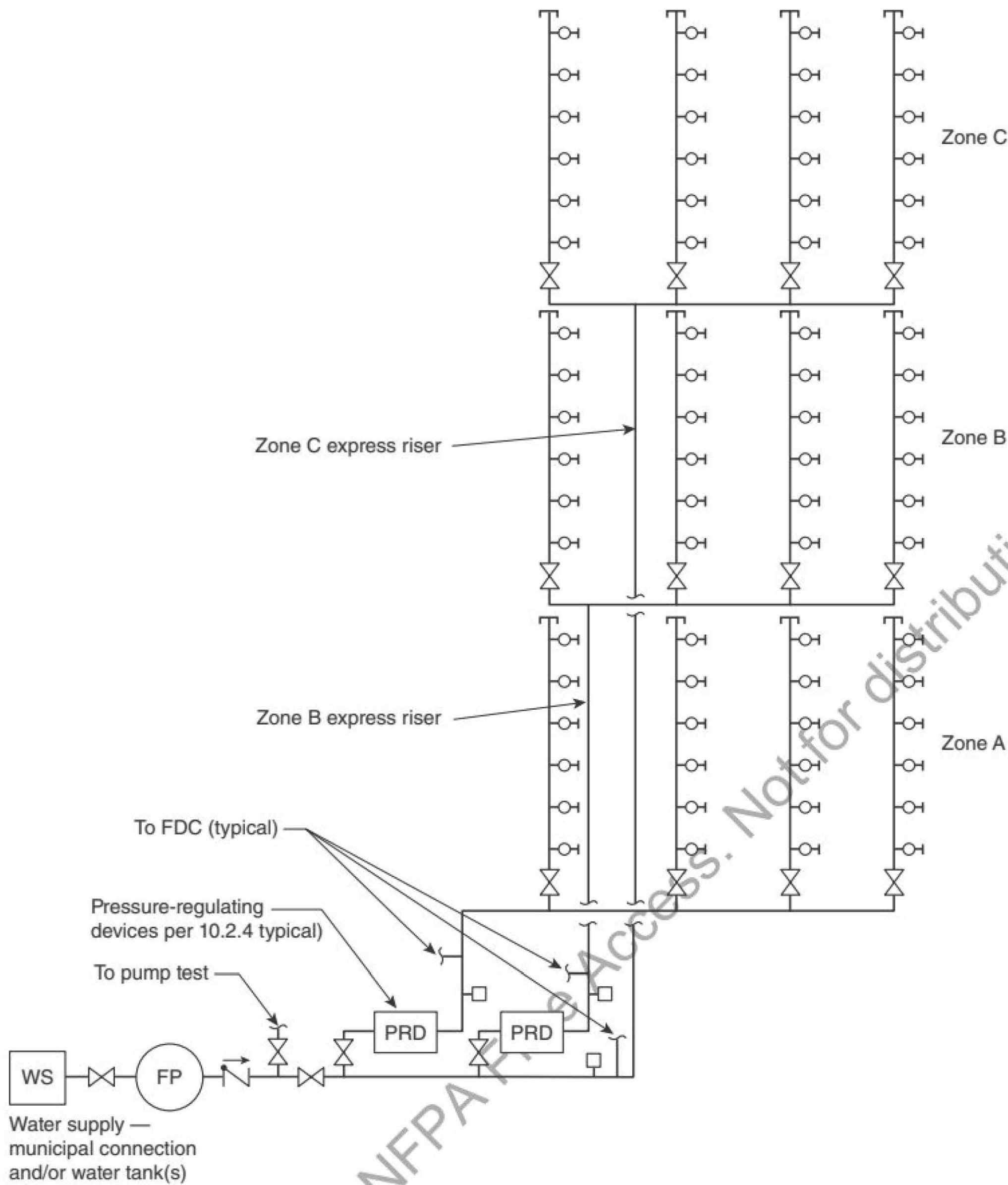
FIGURE A.10.5.2(I) Zones Up to the Level of Fire Department Pumping Capacity Using Pressure-Regulating Devices per 10.2.4 — Three Vertical Standpipe System Zones Example.
