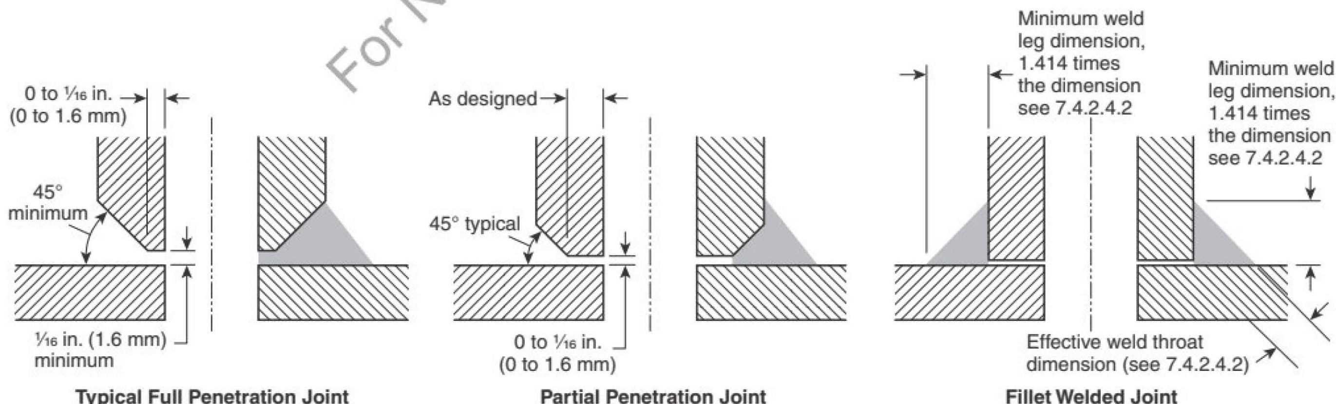
FIGURE A.7.4.2.4.1 Weld Descriptions. [13:Figure A.7.5.2.4.1]
