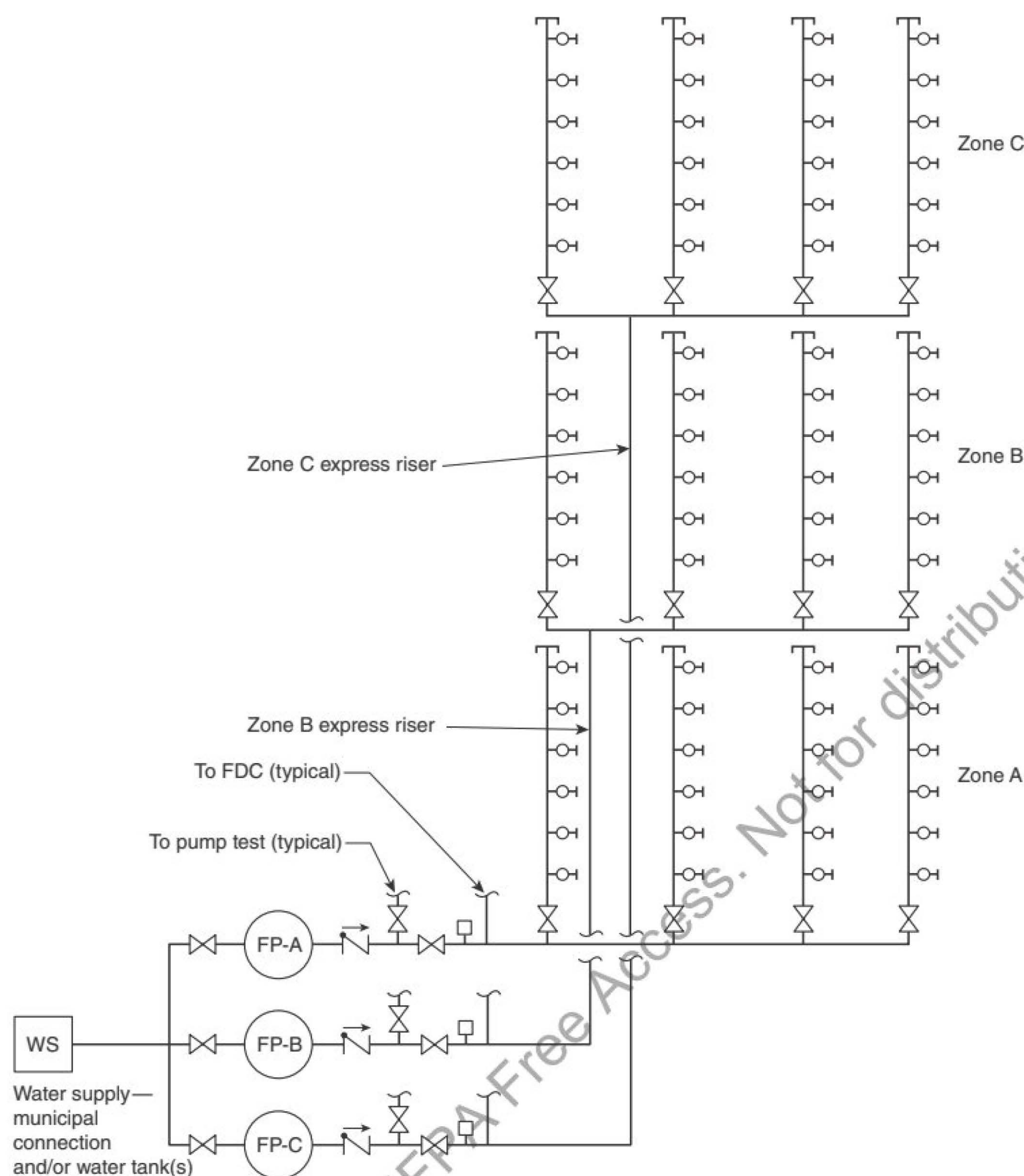
FIGURE A.10.5.2(d) Zones Up to the Level of Fire Department Pumping Capacity Using Separate Pump per Vertical Standpipe System Zone — Three Vertical Standpipe System Zones Example.
