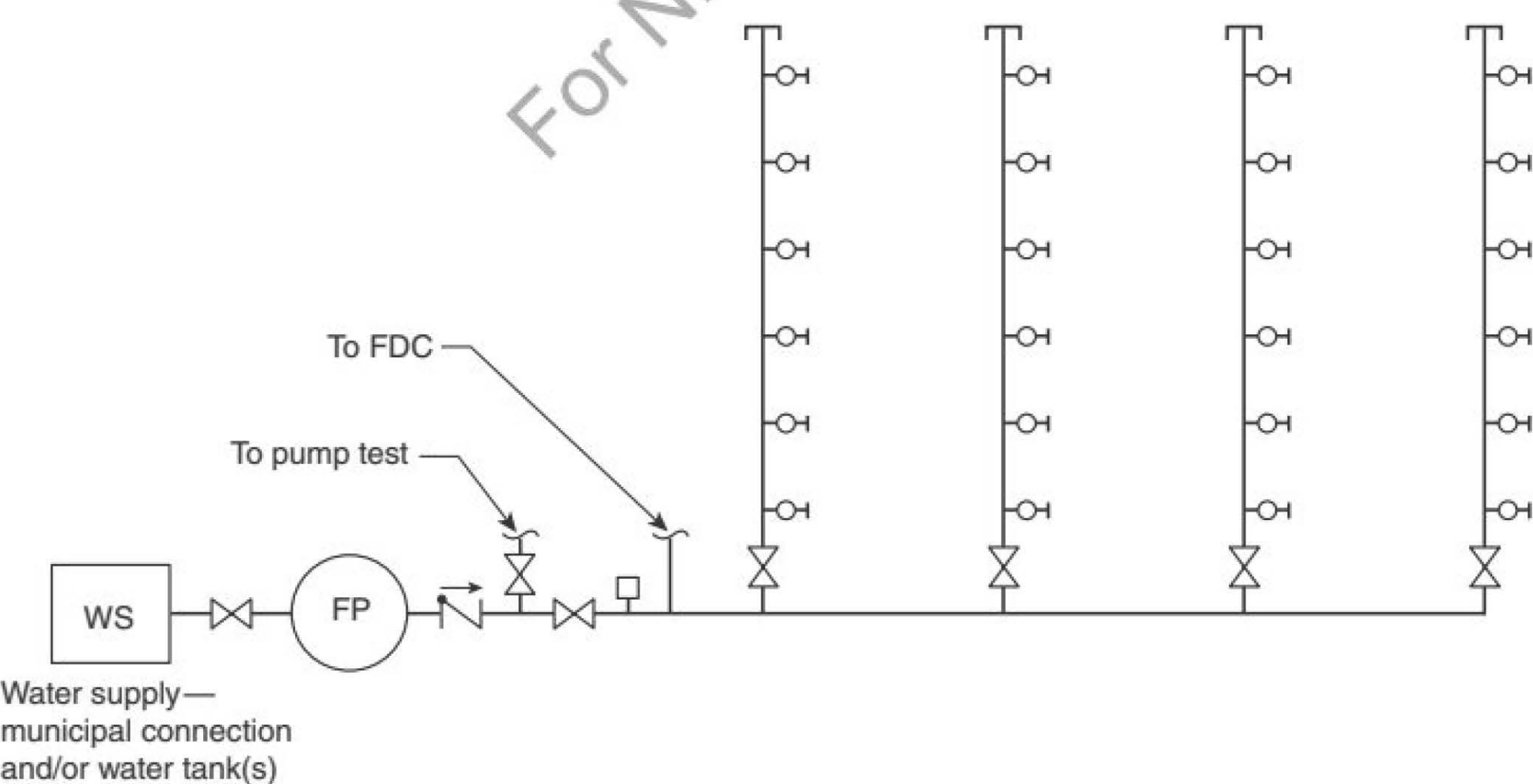
FIGURE A.10.5.2(a) Zones Up to the Level of Fire Department Pumping Capacity — Single Vertical Standpipe System Zone Example.
