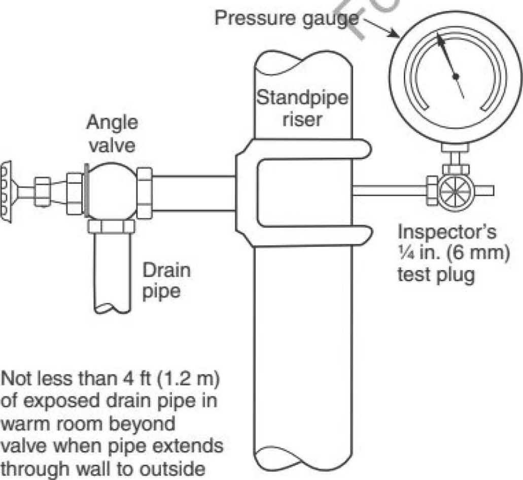
FIGURE 9.10.2.1 Drain Connection for System Riser.
