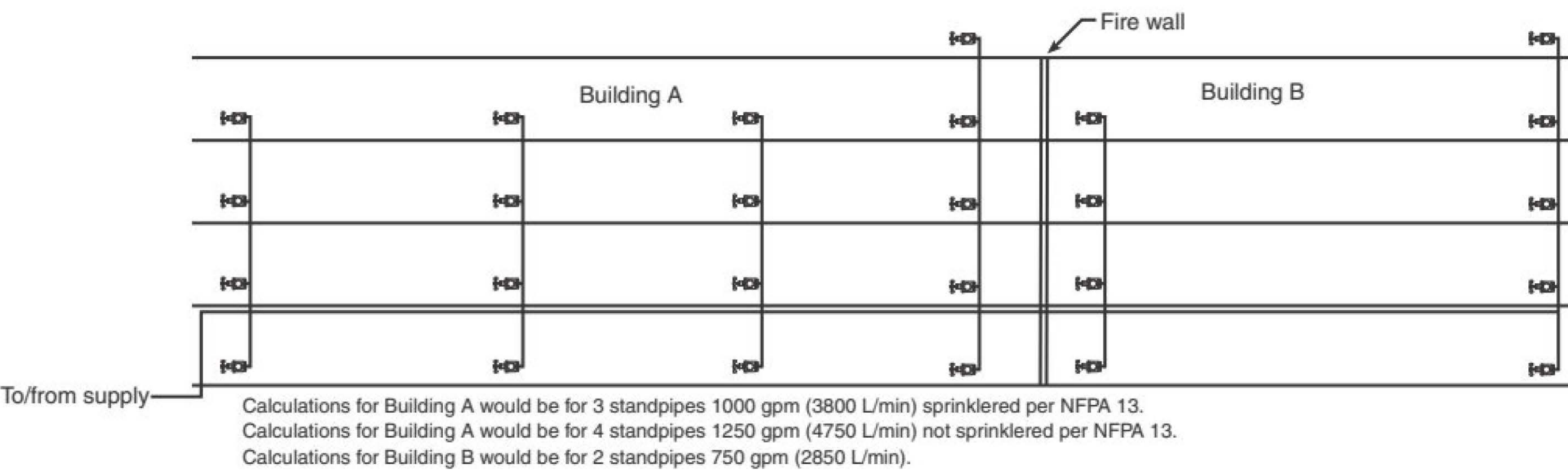
FIGURE A.10.6.1.2.3.1 Common Supply Piping Standpipes Calculated.
