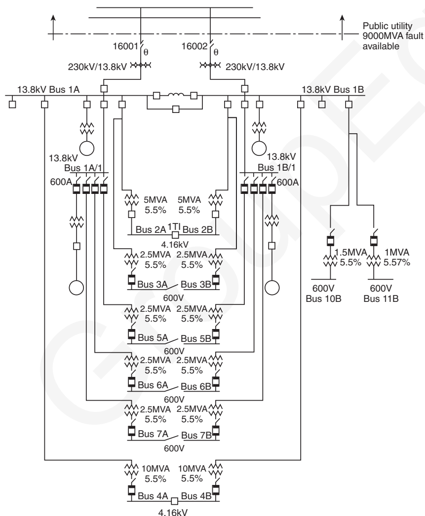
Δ FIGURE D.2.2 Single-Line Diagram of a Typical Petrochemical Complex.
