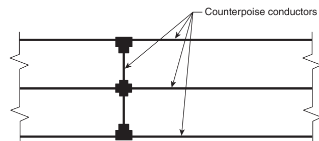
FIGURE 11.4.3.3 Multiple Counterpoise Conductor Installation Interconnection — Plan View.
