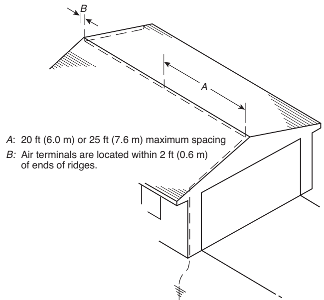
FIGURE 4.7.2.1 Air Terminals on a Pitched Roof.
